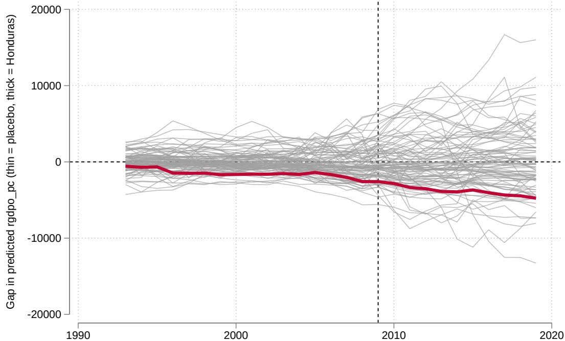
World: factors_yrs (outliers excluded)
